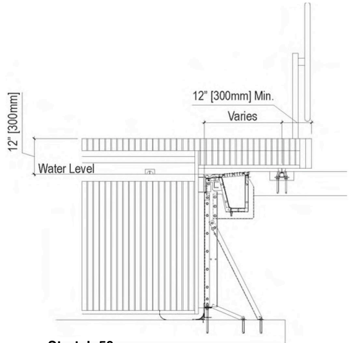
View of Twin Bulkheads across Stretch 50
